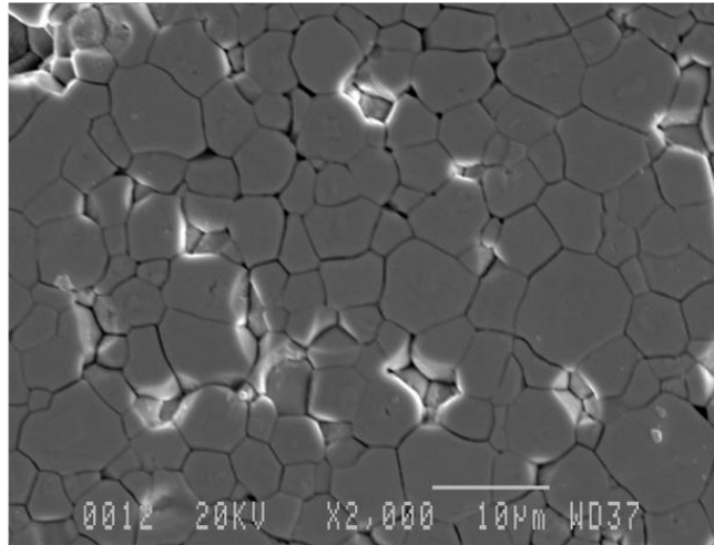
Microstructure of Pz59 at a magnification of 2000 times
