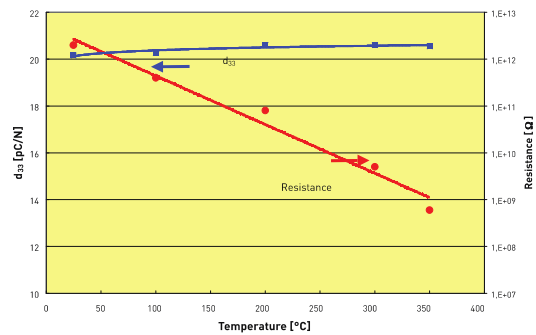
Piezoelectric charge constant and an example of the resistance in a standard disc as a function of temperature. Very low temperature dependencies can be observed.
