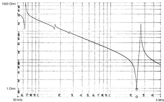
Impedance plot for a circular Pz37 disc. Dimensions are OD25 mm TH 0.5mm. The frequency sweep is from 50 kHz to 5 MHz. The disc shows a planar resonance at approximately 65 kHz, with a planar coupling coefficient, k_p , of only 25%. The thickness resonance at approximately 2300 kHz with a coupling factor, k_t , of 51%.
