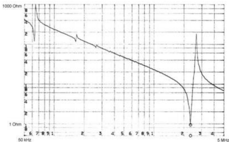
Impedance plot for a circular Pz37 disc. Dimensions are OD25 mm TH 0.5mm. The frequency sweep is from 50 kHz to 5 MHz. The disc shows a planar resonance at approximately 65 kHz, with a planar coupling coefficient, k_p , of only 25%. The thickness resonance at approximately 2300 kHz with a coupling factor, k_t , of 51%.
