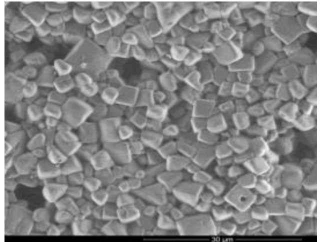
Microstructure of Pz37 at a magnification of 5000 times
